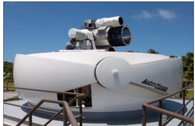
FIGURE 17. The Super RADOT optical sites at Kwajalein are being upgraded with new domes and camera systems.
