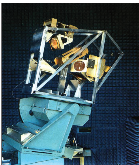
FIGURE 11. The MMW optical beam waveguide is shown being tested in the anechoic chamber at Lincoln Laboratory (left) and after installation on the radar (right).
