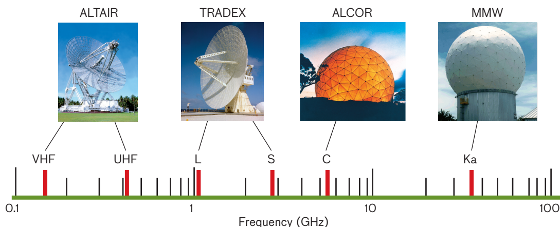
FIGURE 6. The four radars at KREMS utilize the wavebands shown in this simplified frequency scale.
