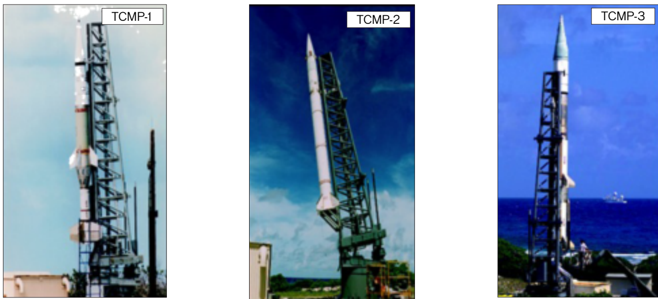
FIGURE 18. Theater Missile Defense (TMD) Critical Measurements Program (TCMP) missiles are launched from Wake Island. Here the missiles await launch on their rails.
