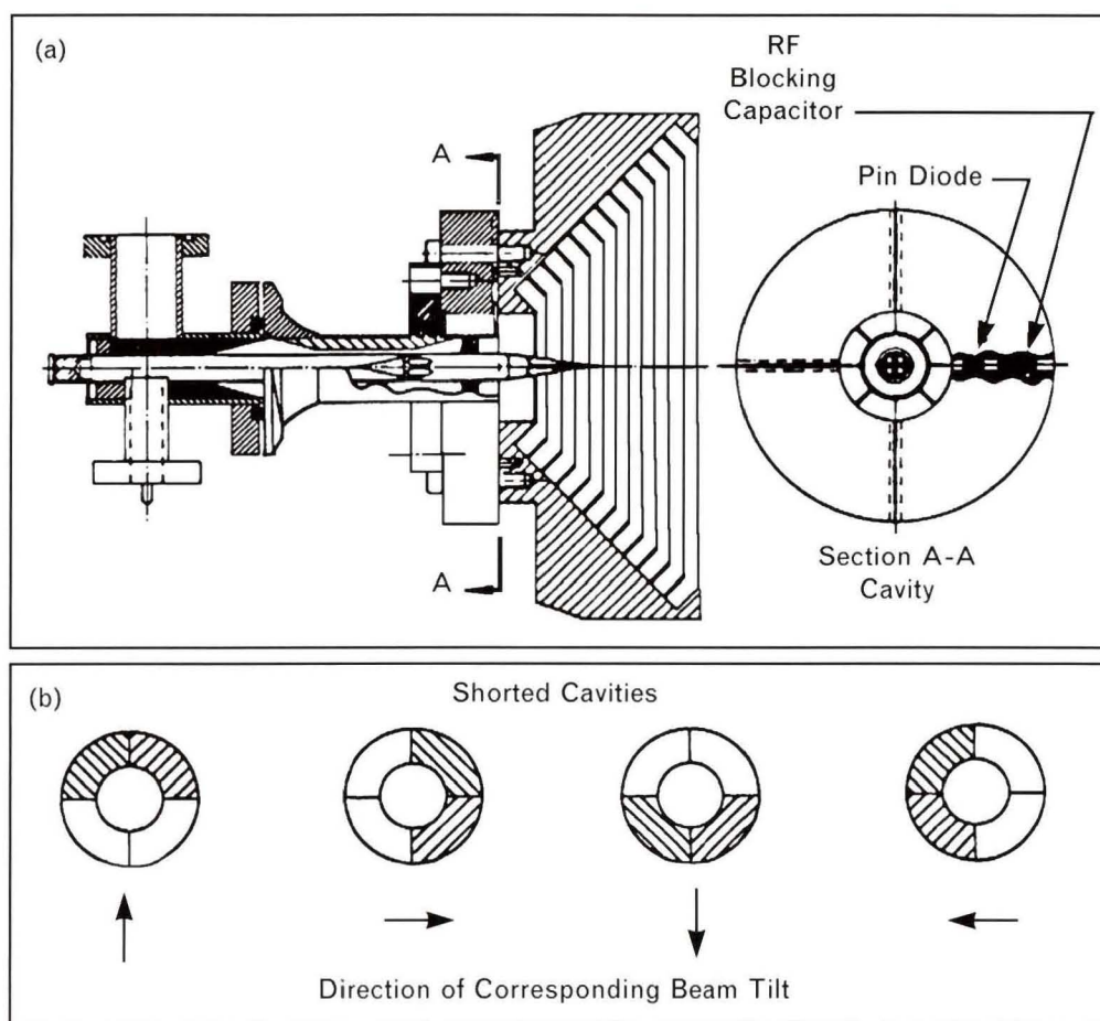
FIGURE 17. Electronic-lobing antenna with diode-switched cavities: (a) sketch of side view and cross section, and (b) diagram showing how switching of the pin diodes displaces the K-band phase center from the reflector focal point. (Note: Shaded areas represent shorted cavities.)
